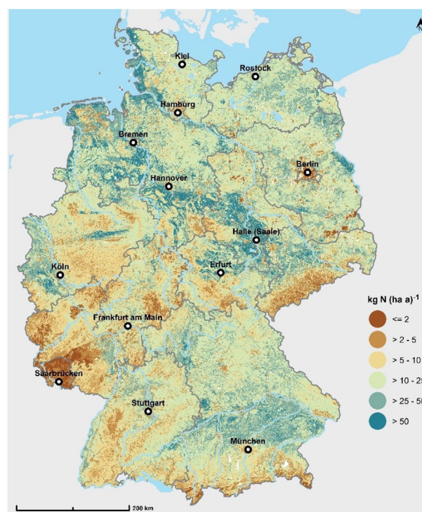
FIGURE 7 Denitrification loss in soil based on displaceable nitrogen input into soil, soil residence time, and maximum denitrification degradation according to the DENUZ model (Wendland et al., 2009).
