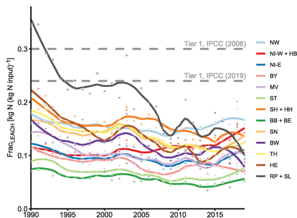
FIGURE 4 GHG inventory time series of Frac_{LEACH} in the study regions compared with IPCC default values (IPCC, 2006, 2019). Points depict modeled annual values for each study region. In order to highlight trends, a curve was fitted using local polynomial regression (LOESS) with a span equal to 0.3.
